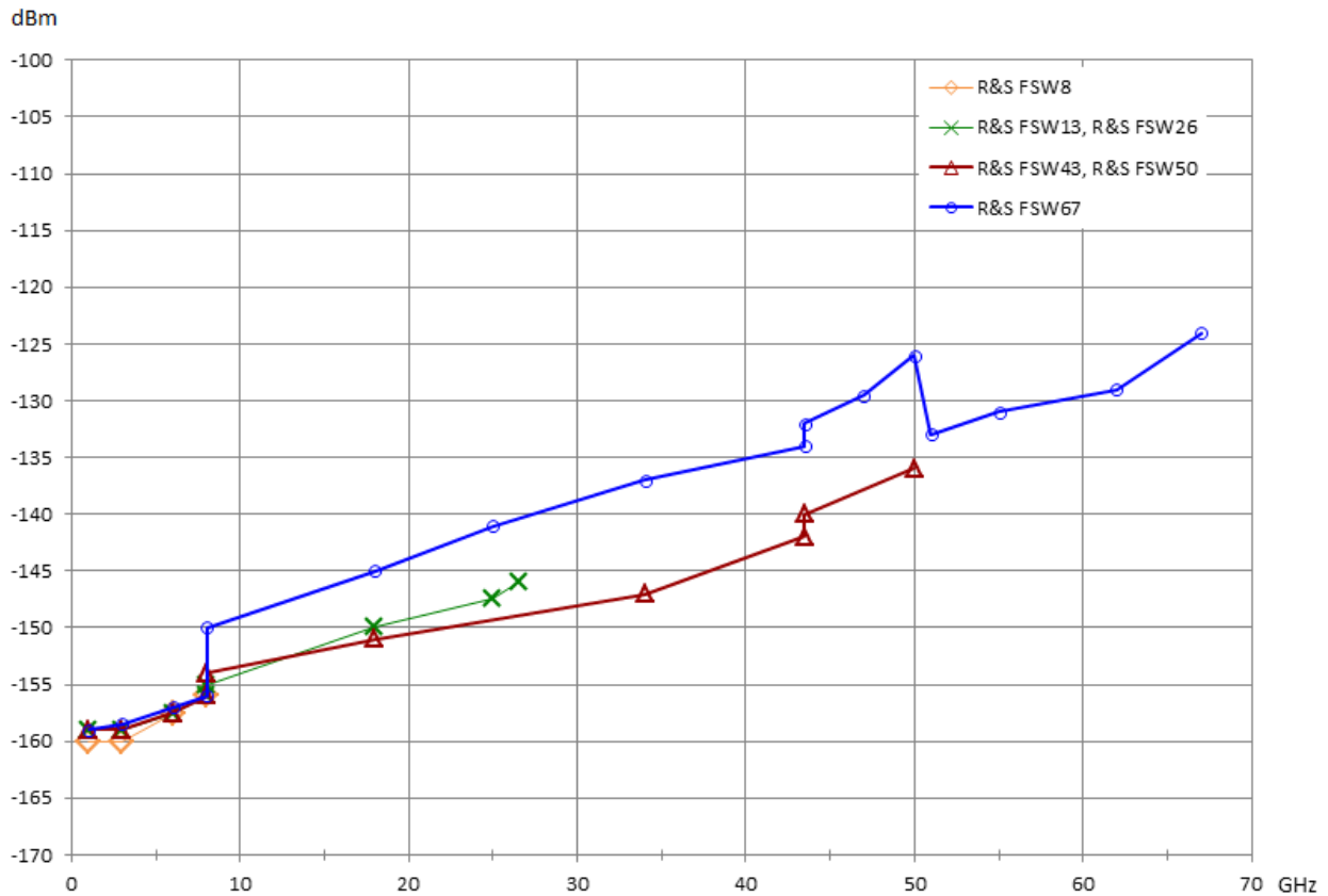
Typical displayed average noise level of the R&S®FSW models for f > 1 GHz without R&S®FSW-B24 RF preamplifier option installed.
